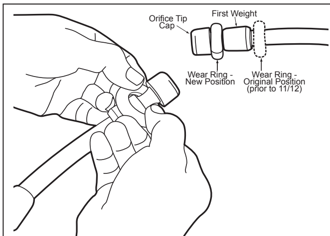
Figure 1. Reposition the First Wear Ring
